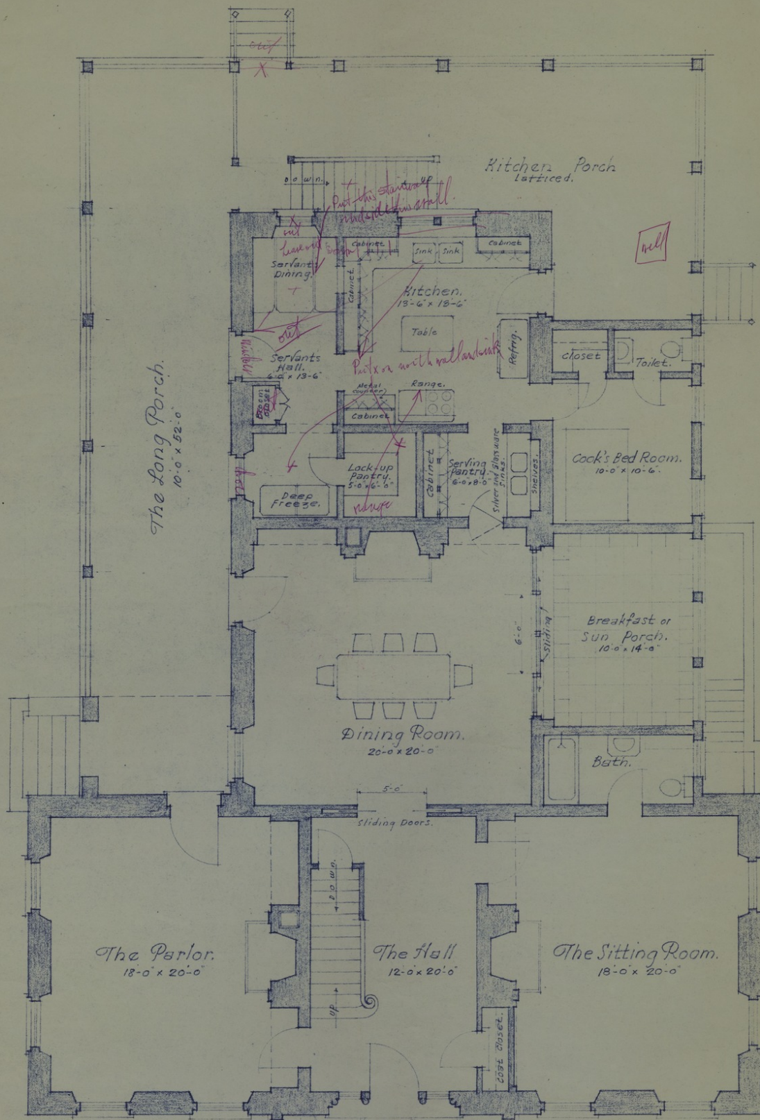
First Floor Plan. Scale \frac{1}{4}'' = 1'-0''
