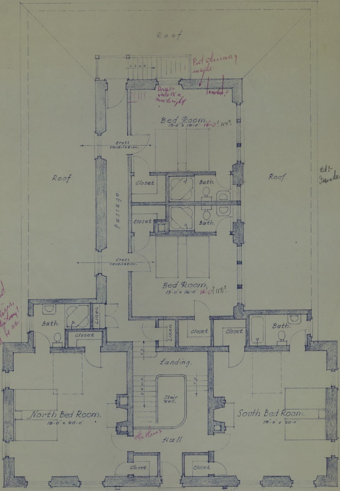
Second Floor Plan. Scale \frac{1}{4}'' = 1'-0''
